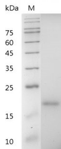
SDS- PAGE analysis of recombinant mouse CXCL12
